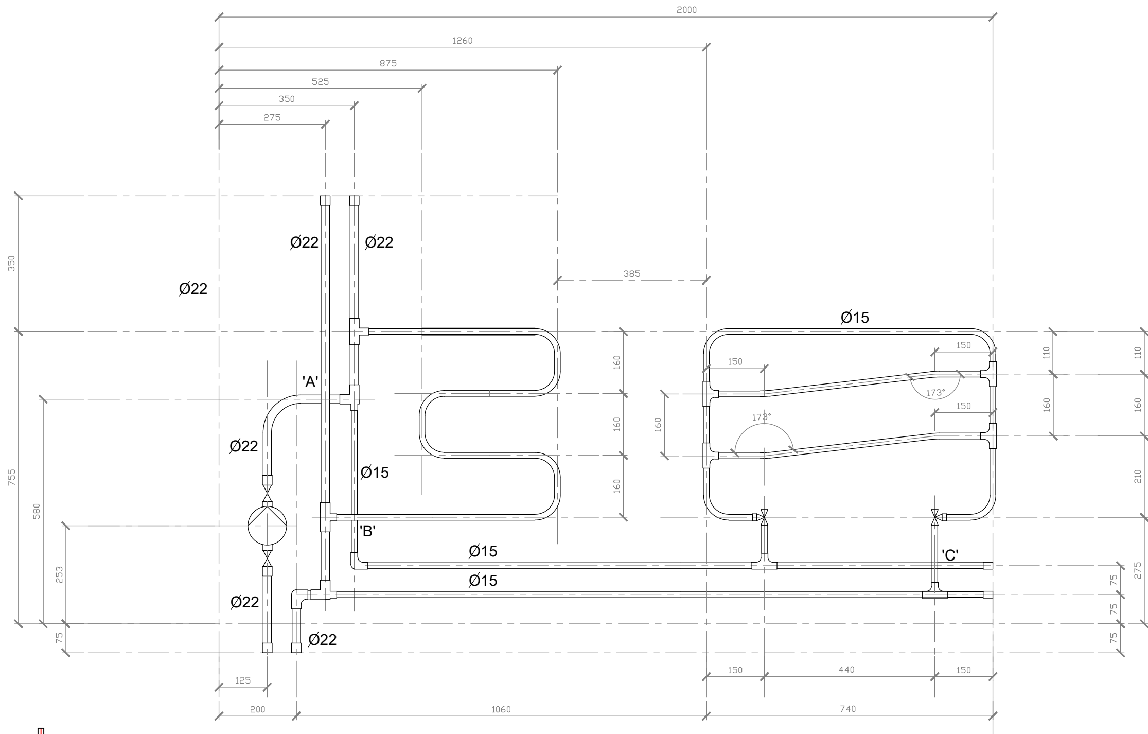
Detail B & C 15mm. Partial Crossover. 15mm clearance
